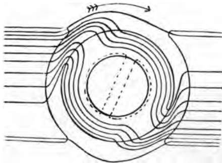
FIG. 237.—Diagram of the Distortion of the Lines of Magnetic Force as they pass through the Body of a Rotating Dynamo Armature.
